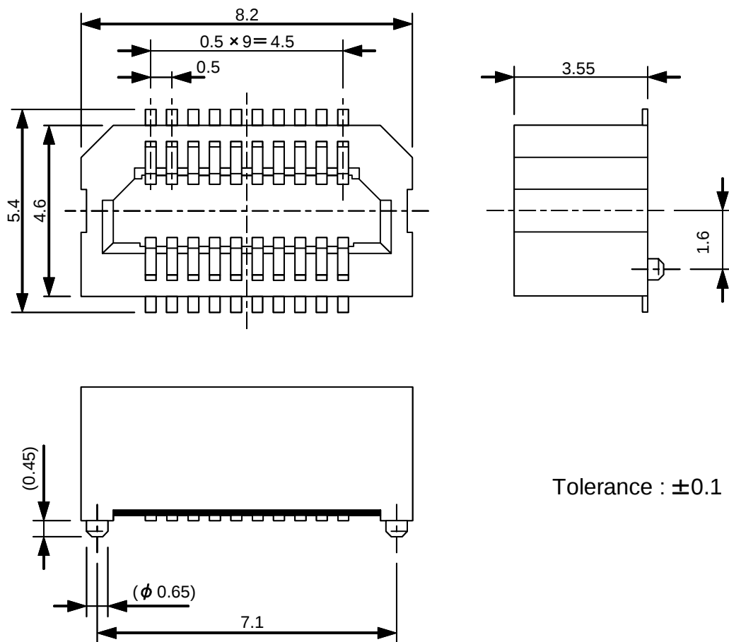
Figure 2.10.7 Drawing of SICAP20S
