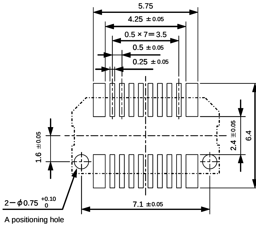
Figure 2.10.8 Recommended pattern of SICA2P20S
